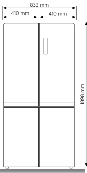
Vista Frontal
